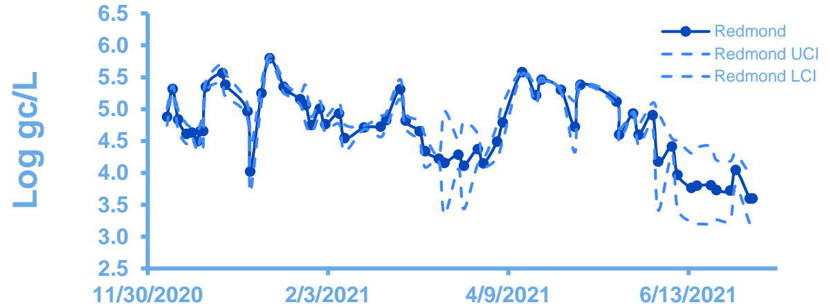
Redmond Wastewater Influent 11/30/20-07/06/21 (Dashed lines = 95% Confidence Intervals)
